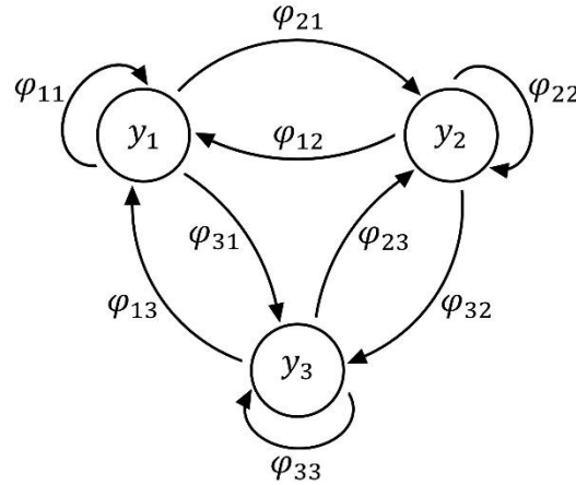
Figure 4: Example of a directed network with three nodes and six unidirectional edges. The nodes of the network consist of three variables y_1 , y_2 , and y_3 . The strength of the lagged associations between these variables is estimated by using the auto- and cross-regressive effects that reside in the transition matrix \Phi of a VAR model.
